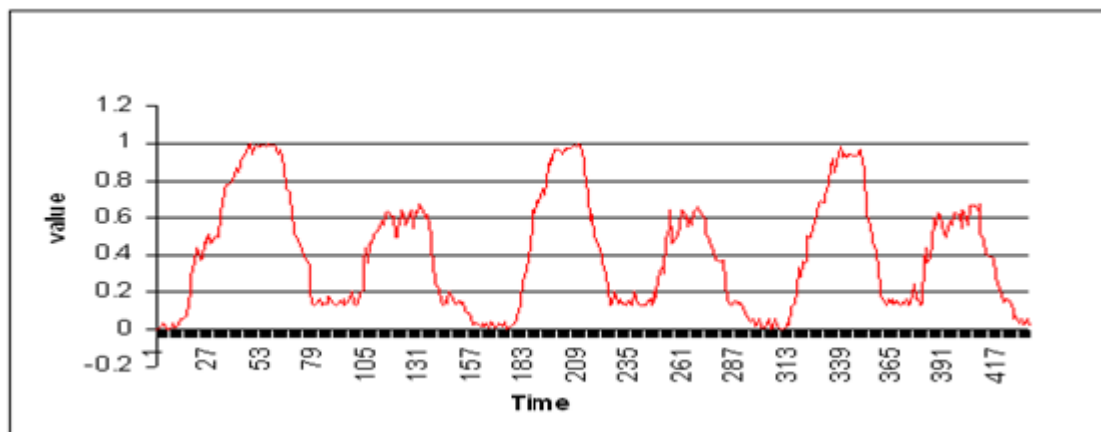
Fig. 1: wkb
